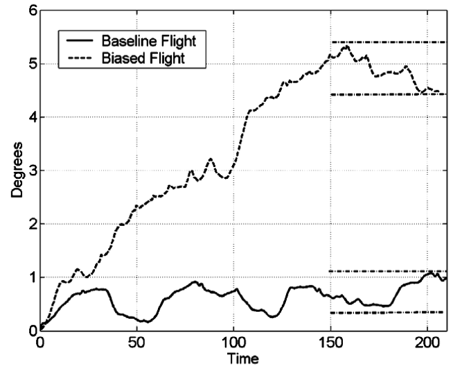
Fig. 8 VS elevator bias estimation.
